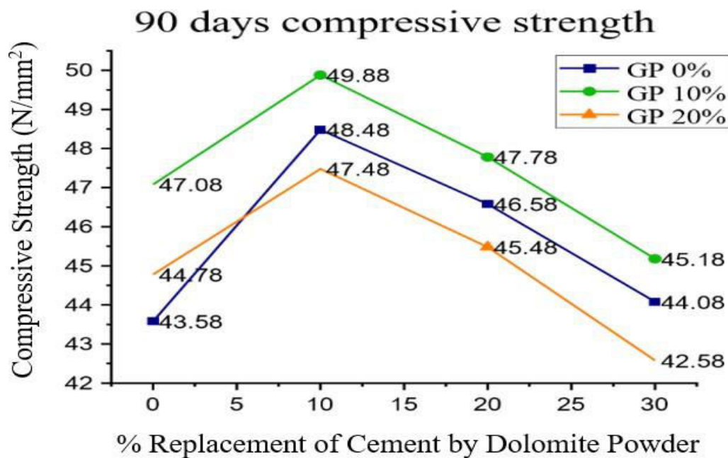
FigureNo2. Variation of Compressive strength at 90days curing
