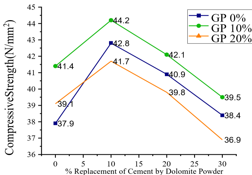
Figure No1. Variation of Compressive strength at 28days curing
