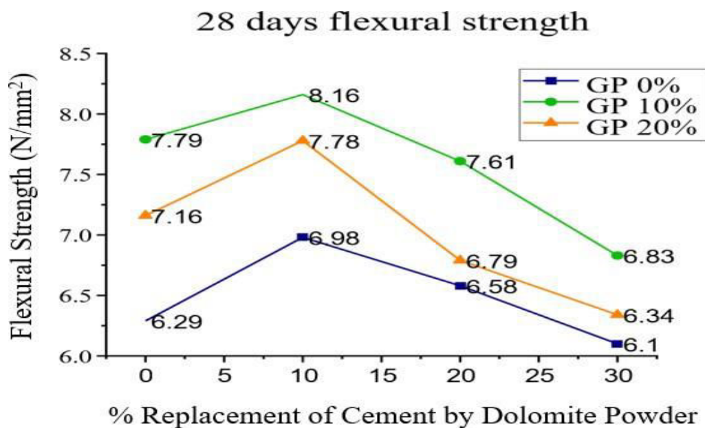
Figure No4. Variation of Flexural strength at 28 days curing
